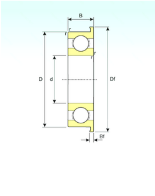
F608 Bearing 2D drawings and 3D CAD models
