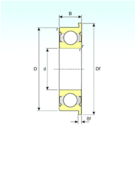
F608ZZ Bearing 2D drawings and 3D CAD models
